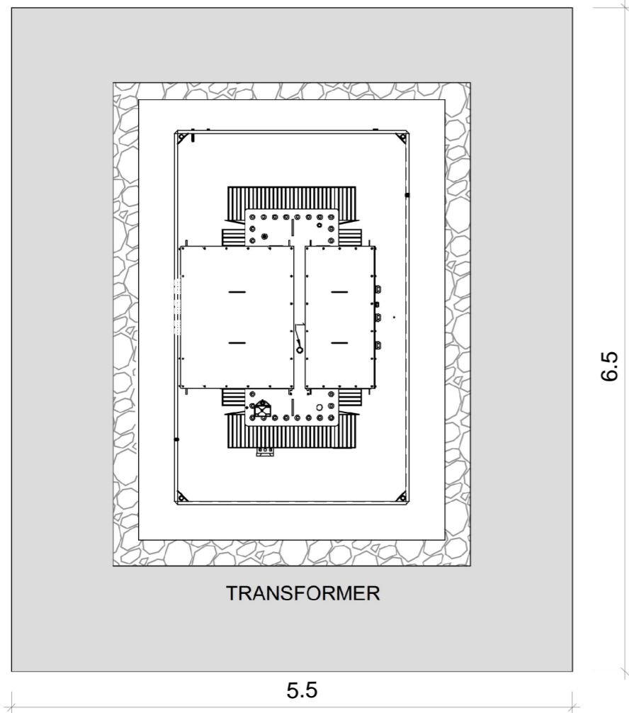
FOOTPRINT Scale 1:50
